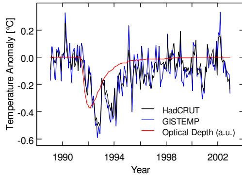
Fig 4 The temperature response to the Pinatubo volcanic eruption in 1991, obtained by removing ENSO and solar responses from the temperature records of HadCRUT and GISTEMP. The red line shows (in arbitrary units) the estimated time course of the stratospheric optical density resulting from the volcano's aerosol (Sato et al 1993)
