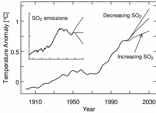
Fig 9 Extrapolation of the model to the year 2030. Greenhouse gas forcing after 2010 is linearly extrapolated based on the 2001-2010 trend, solar forcing is assumed to remain constant at the mean 1950-2010 level, and SO 2 forcing is computed for three scenarios (see inset), either with decreasing SO 2 (2006-2010 at the 2005 level, followed by a yearly decrease of 2.5 \cdot 10^3 Gg SO 2 /year), constant SO 2 (2006-2030 remaining at the 2005 level), or increasing SO 2 (2006-2010 rising at the 2002-2005 rate, followed by a yearly increase of 2.5 \cdot 10^3 Gg SO 2 /year). The two axes of the inset encompass the years 1900-2030 and emissions of 0-2 \cdot 10^5 Gg SO 2 /year, respectively
