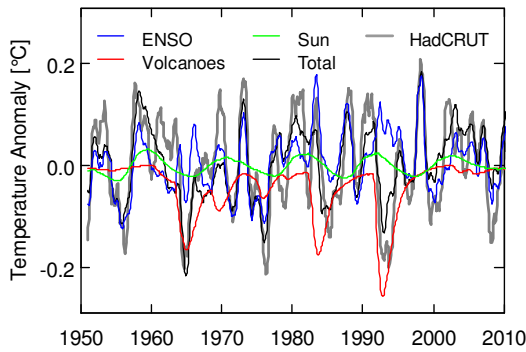
Fig 2 Fit to the measured average global temperature (HadCRUT3) for the years 1951-2010, with forcings attributable to ENSO (El Niño Southern Oscillation), stratospheric aerosol originating from volcanic eruptions, and solar irradiance cycles. Temperature and solar irradiance were detrended with a loess polynomial fit before fitting, and ENSO, volcanic, and solar forcings were low-pass filtered as part of the fit
