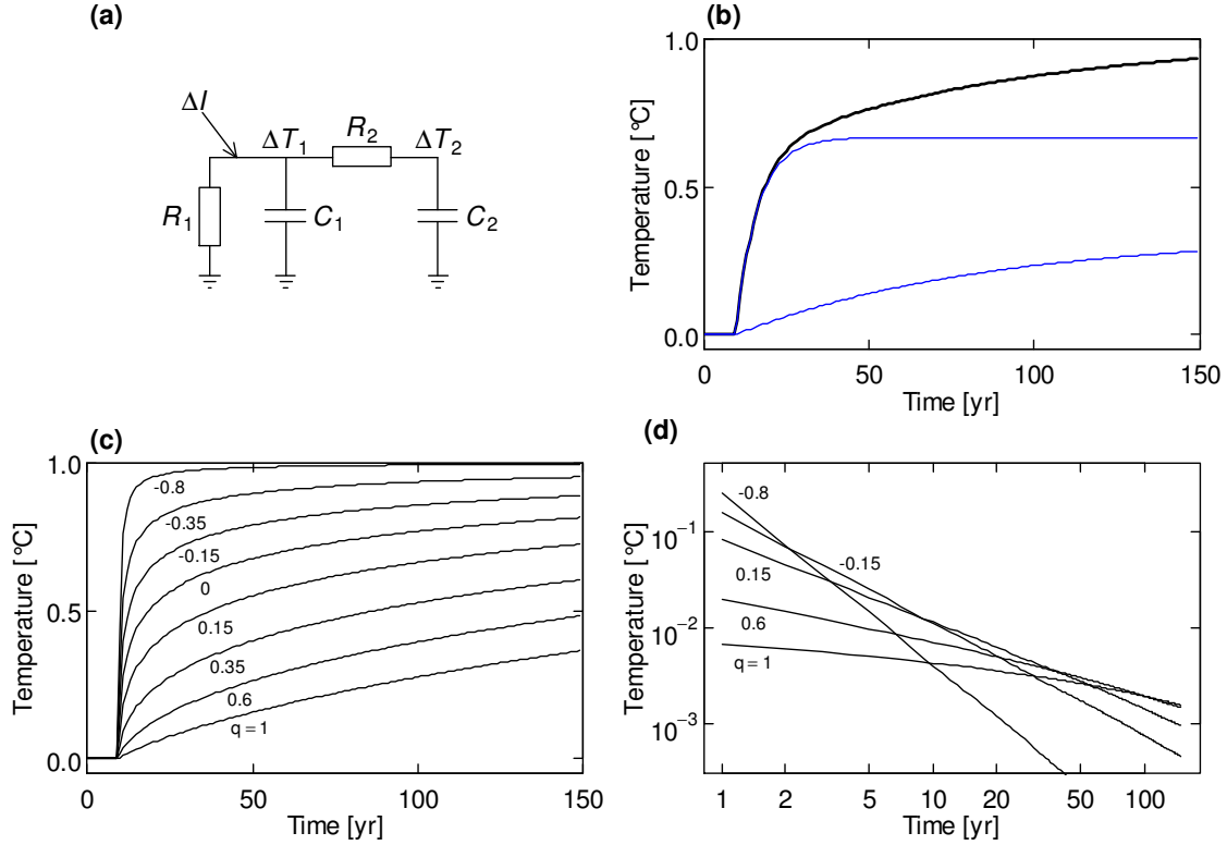
Fig. 1 a Equivalent circuit for a simple model of global temperature change \Delta T_1 in response to a forcing \Delta I . C_1 and C_2 represent the heat capacities of the ocean upper mixed layer and a deeper layer, respectively, R_2 the resistance to heat flowing between these two layers, and R_1 the resistance to heat radiating to space. See text for further explanation. b Black line: example response \Delta T_1 of the circuit in a to a step \Delta I=1 \text{ Wm}^{-2} , with R_1=1 \text{ K}/(\text{Wm}^{-2}) , R_2=2 \text{ K}/(\text{Wm}^{-2}) , C_1=10 \text{ Jm}^{-2}/\text{K} , and C_2=25 \text{ Jm}^{-2}/\text{K} . The response can be approximated by two exponential curves (blue lines). See text for further explanation. c Fractal climate response functions according to Eq. 4 with n=6 . All curves go asymptotically to 1, but do so with different weightings of the six composing exponential curves (with e -folding times of 0.5, 2, 8, 32, 128, and 512 years). d Fractal climate pulse responses according to Eq. 1. The axes are both logarithmic, thus the approximately straight lines show power-law (fractal) scaling
