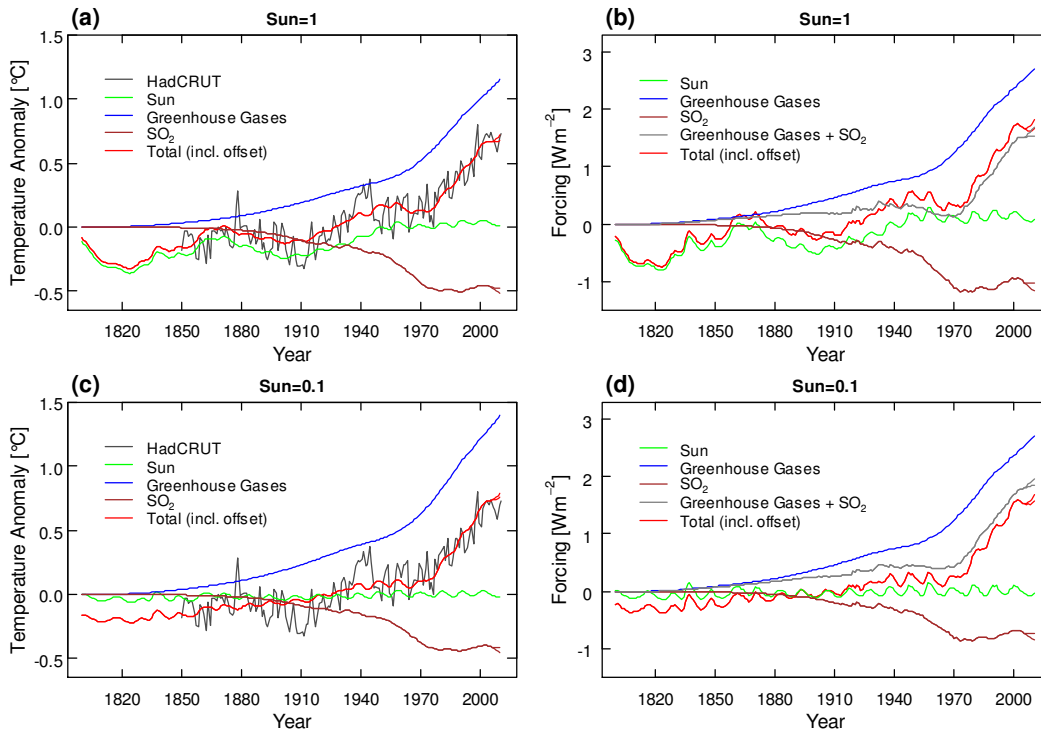
Fig 7 Analysis of the contribution of the various forcings to the model as fitted to the modern temperature trend. The fit in a is identical to the one in Fig. 5d, thus made to HadCRUT and GISTEMP simultaneously, but only HadCRUT is shown here for the sake of clarity. The total temperature in a includes an offset of 0.03 °C. The forcings corresponding to the temperature responses in a are shown in b , where the total includes an offset of 0.06 Wm -2 . In c and d the results are shown when the fit is made with a solar irradiance with tenfold-reduced modulations (apart from the solar cycles, which are left intact). Totals include offsets of -0.16 °C and -0.24 Wm -2
