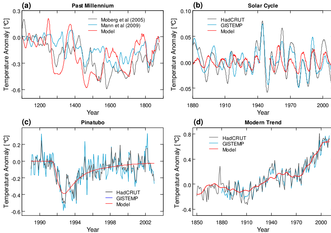
Fig 5 The response of the model of Eq. 1 to forcings attributable to solar irradiance, greenhouse gases, and \text{SO}_2 -related aerosol (see text and Section 2 for details), as fitted simultaneously to the four types of temperature records shown in a-d . In a the reconstructions of temperatures of the past millennium made by Moberg et al (2005) and Mann et al (2009) are shown, in b the response to solar cycles isolated from the HadCRUT and GISTEMP temperature records (as in Fig. 3), in c the response to the Pinatubo eruption (as in Fig. 4), and in d the modern temperature trends from HadCRUT (1850-2010) and GISTEMP (1880-2010). Anomalies of the measured temperatures in a and d are given relative to the mean temperature of 1880-1970
